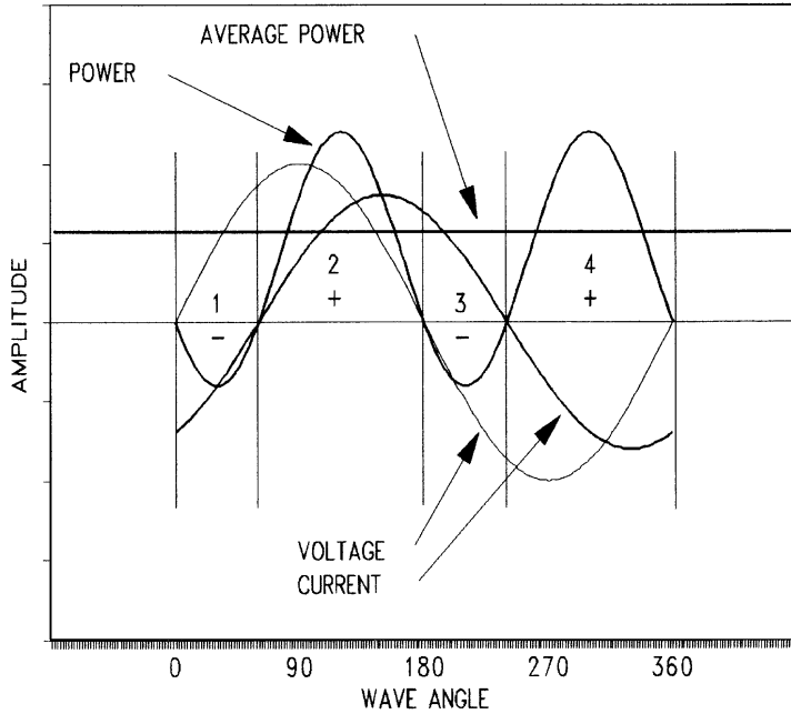
FIGURE 40.4 Voltage, current, and power for sine waves 60° out of phase. The vertical scales for voltage and current amplitudes are the same as those for Figure 40.3. Current lags voltage by 60° and both are sinusoidal. The power is positive in regions (2) and (4), and negative in regions (1) and (3). Average power delivered to do work is less than the maximum power.
