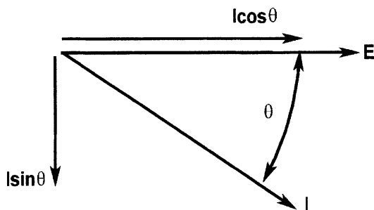
FIGURE 40.6 Phasor diagram for current and voltage. Voltage is the reference phasor. The current I has been resolved into orthogonal components I\cos\theta and I\sin\theta . (From Reference [1].)
