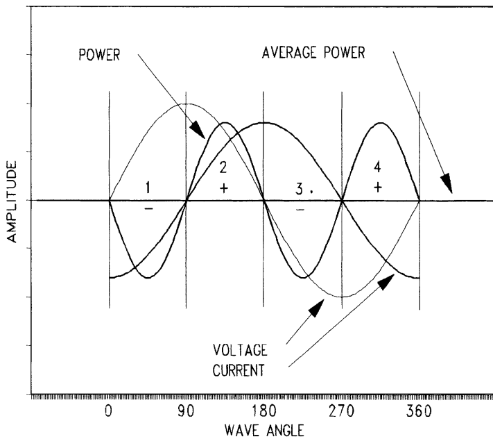
FIGURE 40.5 Voltage, current, and power for sine waves 90° out of phase. The vertical scales for voltage and current amplitudes are the same as those for figure 40.3. Current lags voltage by 90° and both are sinusoidal. The power is positive in regions (2) and (4), negative in regions (1) and (3), and is of equal absolute magnitude in all four regions. Average power delivered to do work is zero.
